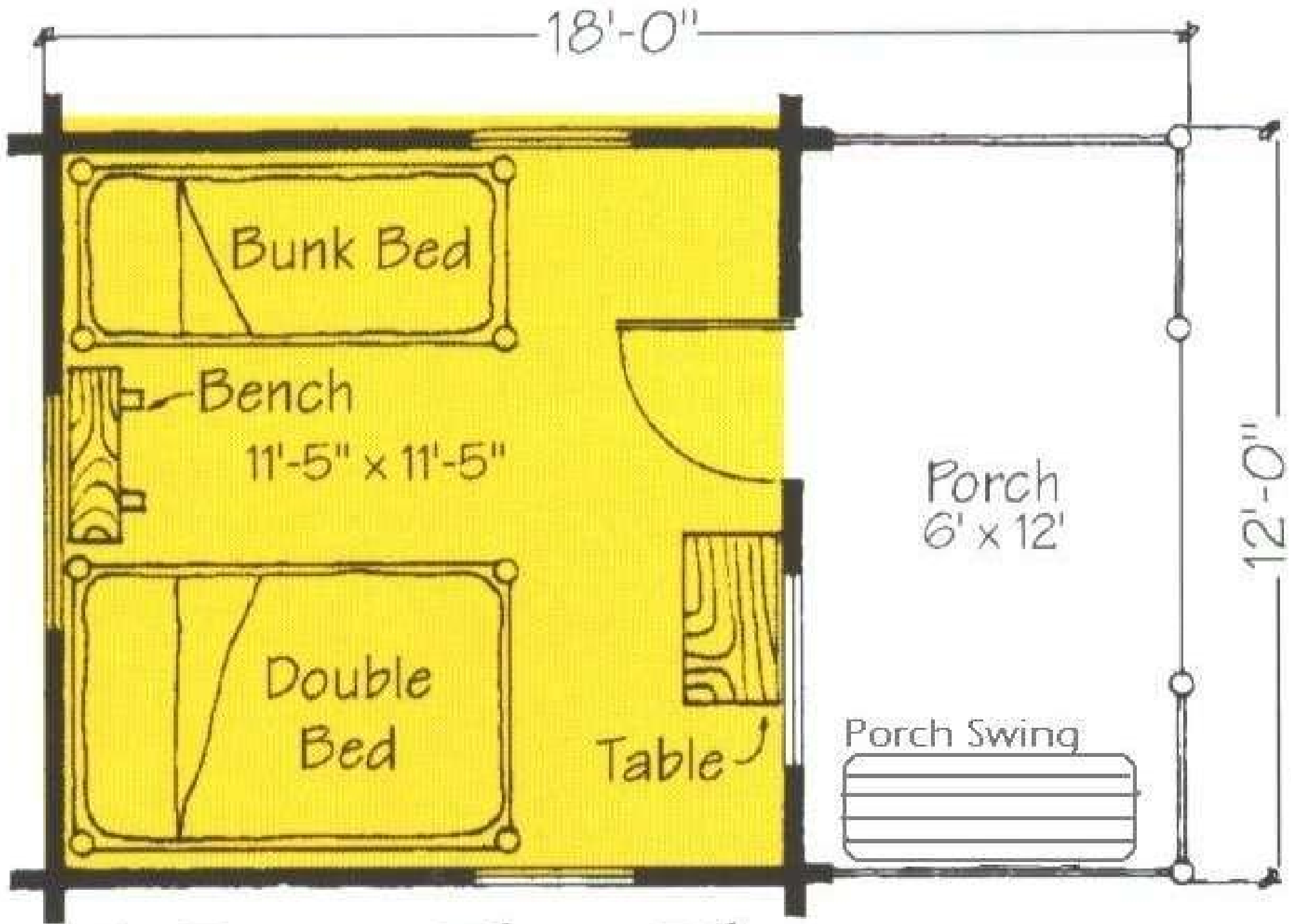
1-Room Floor Plan
